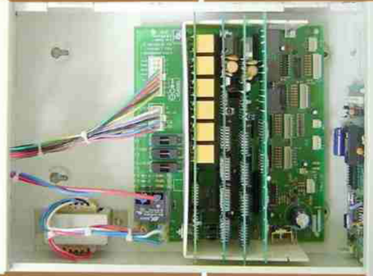
RELAY CONTROL UNIT 330 mm x 110 mm x 230 mm
